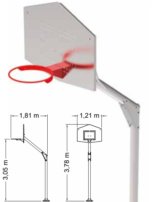
CANASTA BASKET Ref. 81295
