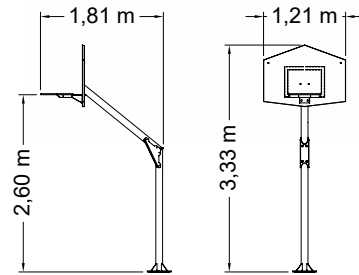
CANASTA MINIBASKET Ref. 80926
